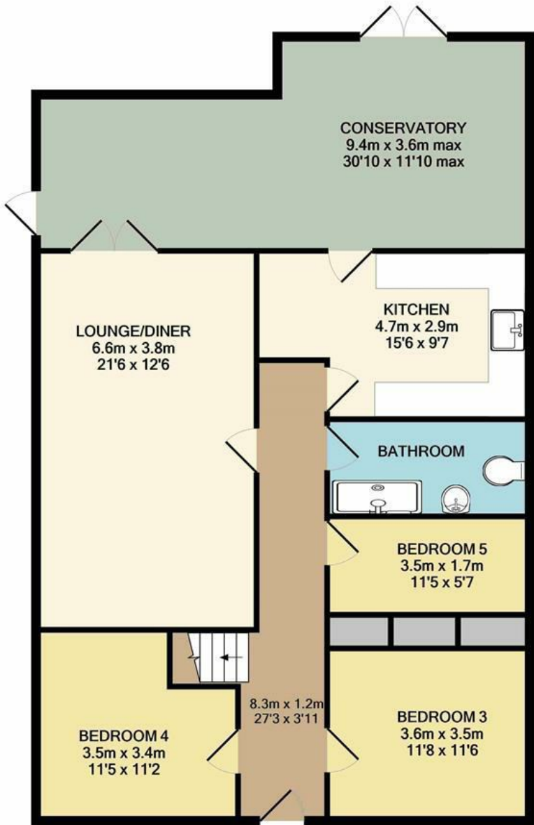
GROUND FLOOR APPROX. FLOOR AREA 111.4 SQ.M. (1199 SQ.FT.)
